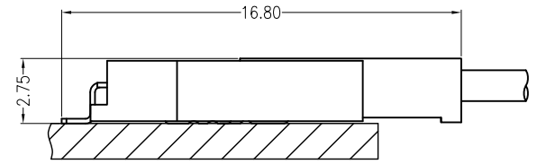
Assembly Layout
