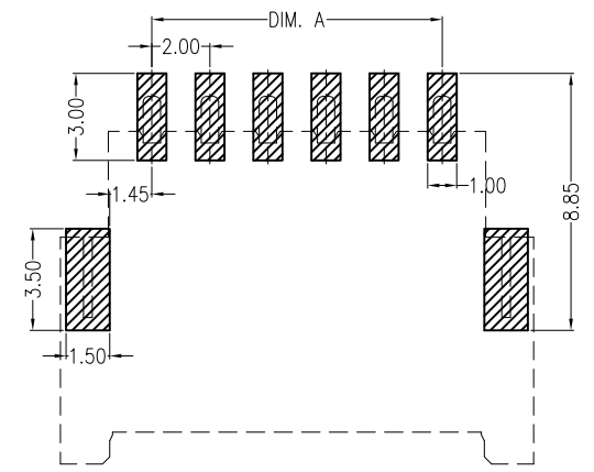
SUGGESTED PCB LAYOUT
